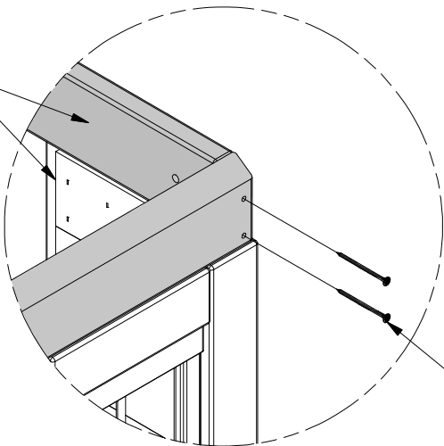
201 (x4) SCREW - 2 1/2"
