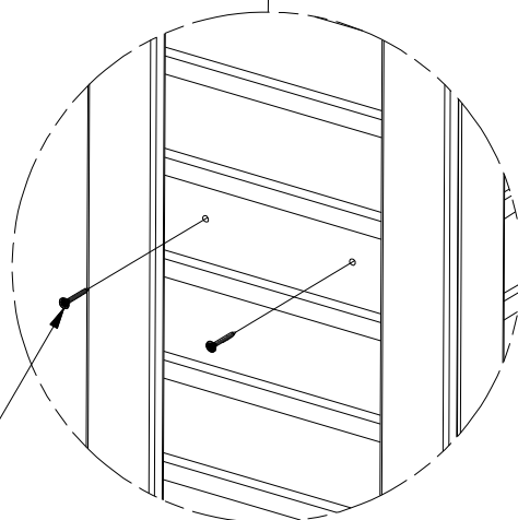
387 (x4) SCREW - 1 1/4"
