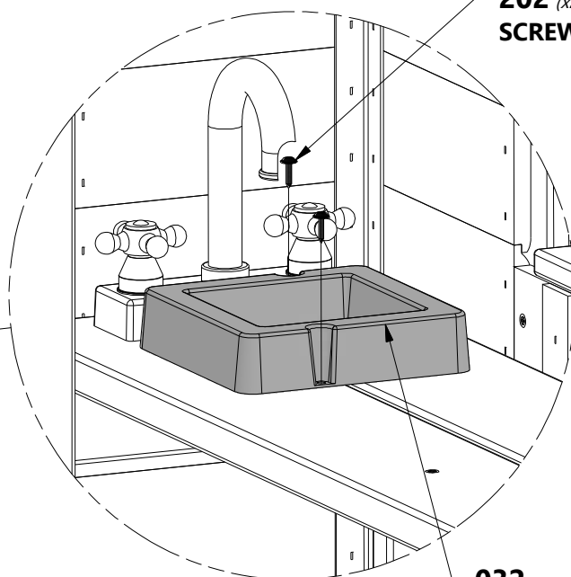
032 (x1) SURFACE MOUNT BASIN
